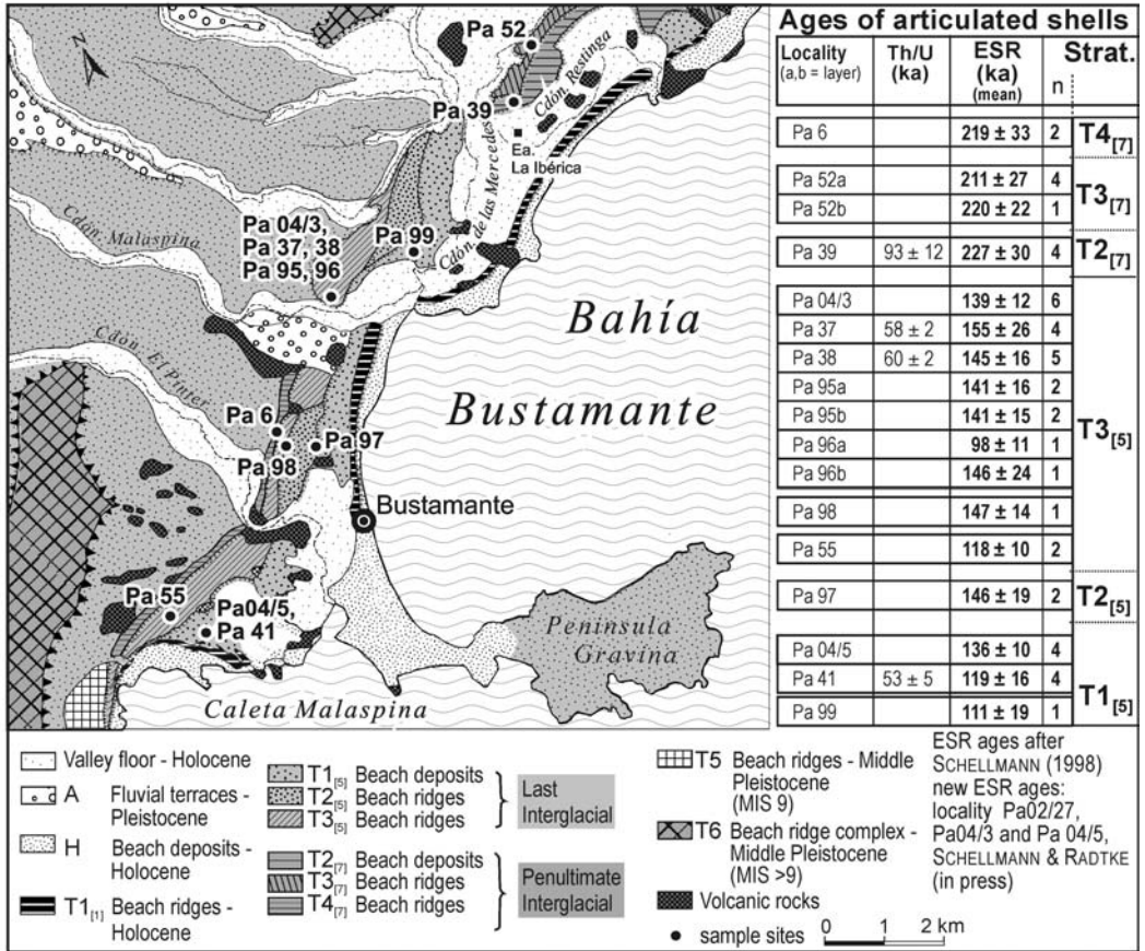
Fig. 7: ESR (mean ages) and TMS Th/U ages of articulated mollusc shells of Last and Penultimate Interglacial beach ridge systems along the Patagonian Atlantic coast near Bustamante. TMS Th/U dating by A. Rostami & A. Mangini (Institut für Umweltphysik, Universität Heidelberg); details in SCHELLMANN (1998) and SCHELLMANN & RADTKE (2000).
