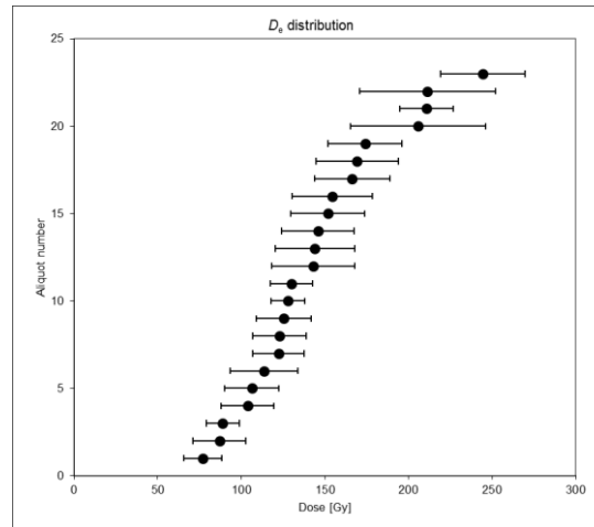
Müb-5 quartz OSL (2 mm aliquots)
