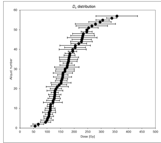
REU-2 quartz OSL (2 mm aliquots)
