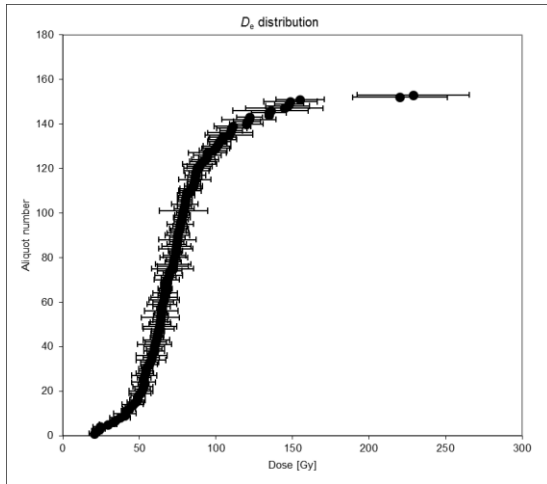
Müb-7 feldspar IR50 (single grains)
