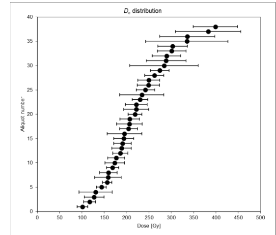
Müb-6 feldspar pIR225 (single grains)
