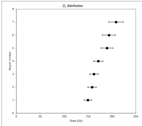
BIR-1 poly IR50 (fine grains)
