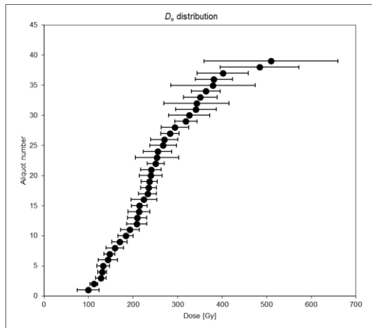
Müb-5 feldspar pIR225 (single grains)
