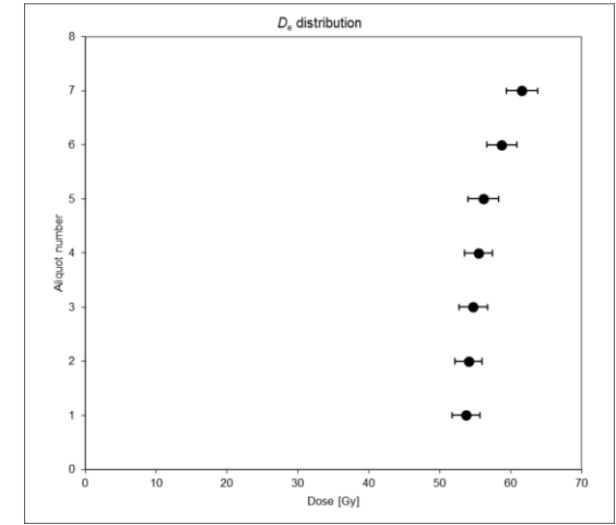
BIR-3 poly IR50 (fine grains)
