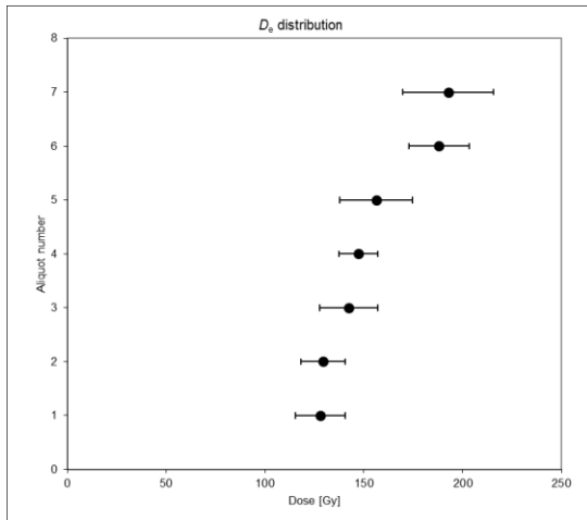
BIR-1 quartz OSL (fine grains)
