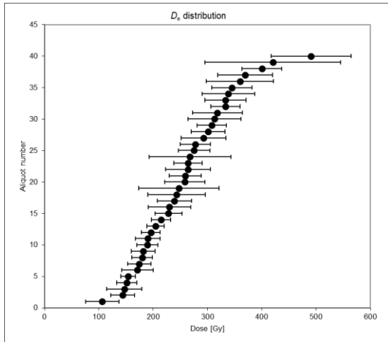
REU-2 feldspar IR50 (single grains)
