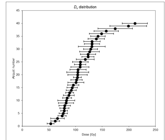
Müb-6 quartz OSL (2 mm aliquots)
