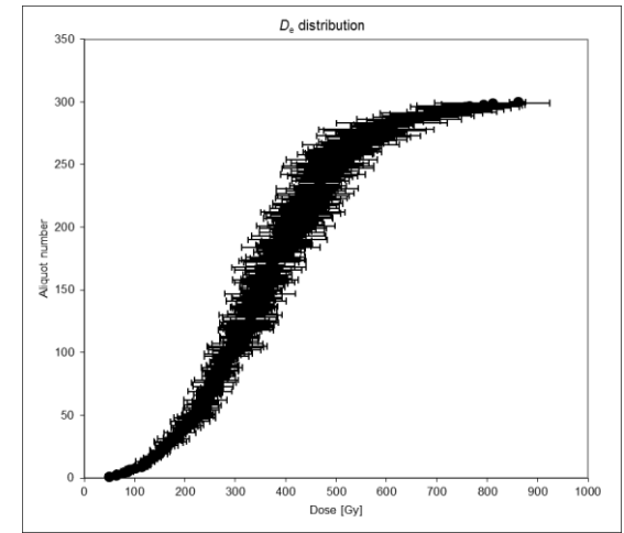
RÜT-1 feldspar IR50 (single grains)
