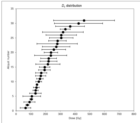
RÜT-1 quartz OSL (single grains)
