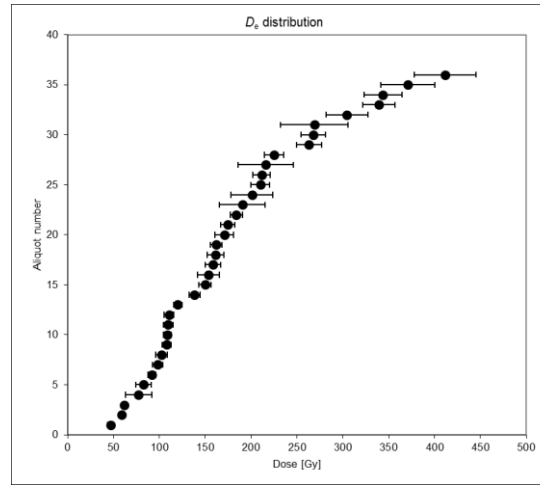
BIR-2 feldspar IR50 (1 mm aliquots)
