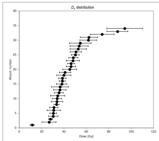
SZB-2 quartz OSL (2 mm aliquots)
