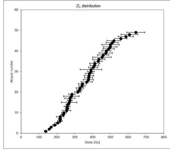
RÜT-1 feldspar IR50 (1 mm aliquots)
