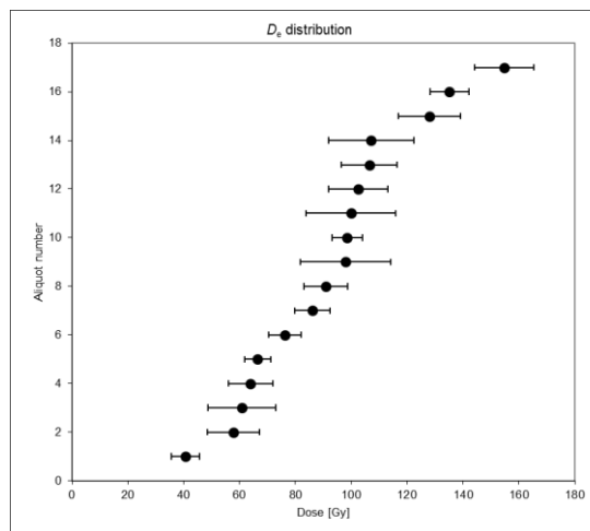
BIR-2 quartz OSL (2 mm aliquots)
