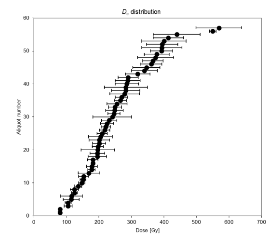
Müb-6 feldspar IR50 (single grains)
