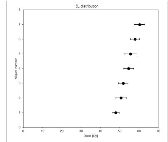
BIR-3 quartz OSL (fine grains)
