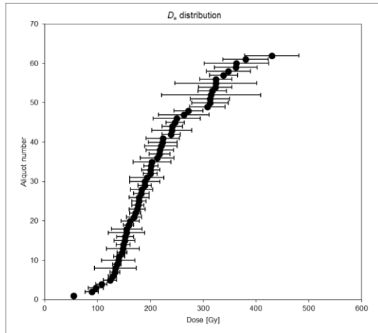
Müb-5 feldspar IR50 (single grains)
