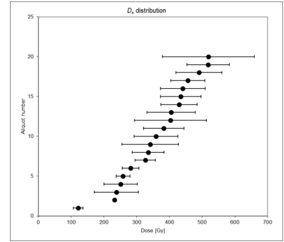
RÜT-1 feldspar pIR225 (single grains)
