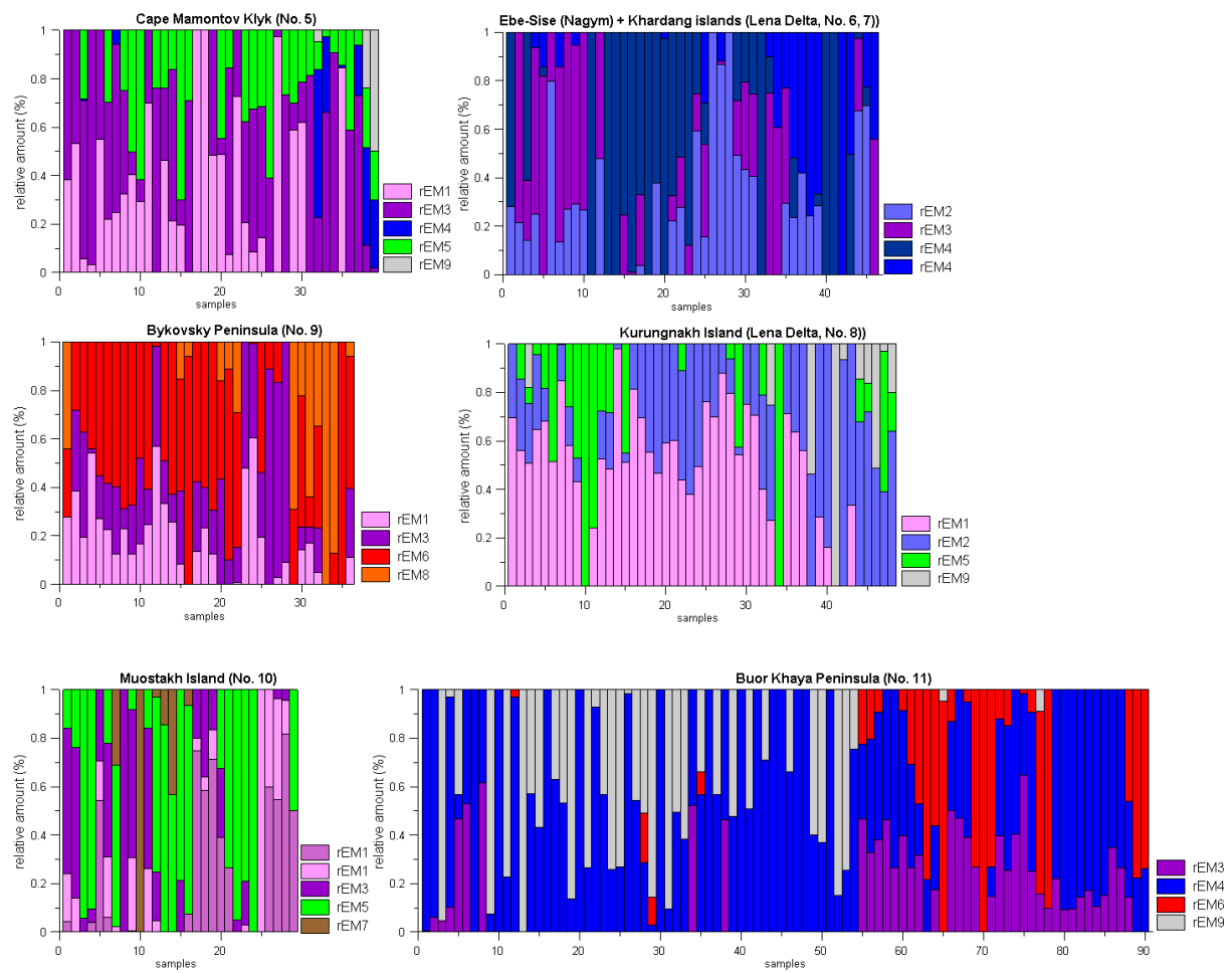
Fig. S5.2 Mean scores from the Laptev Sea coast and the Lena Delta Yedomas sites.
