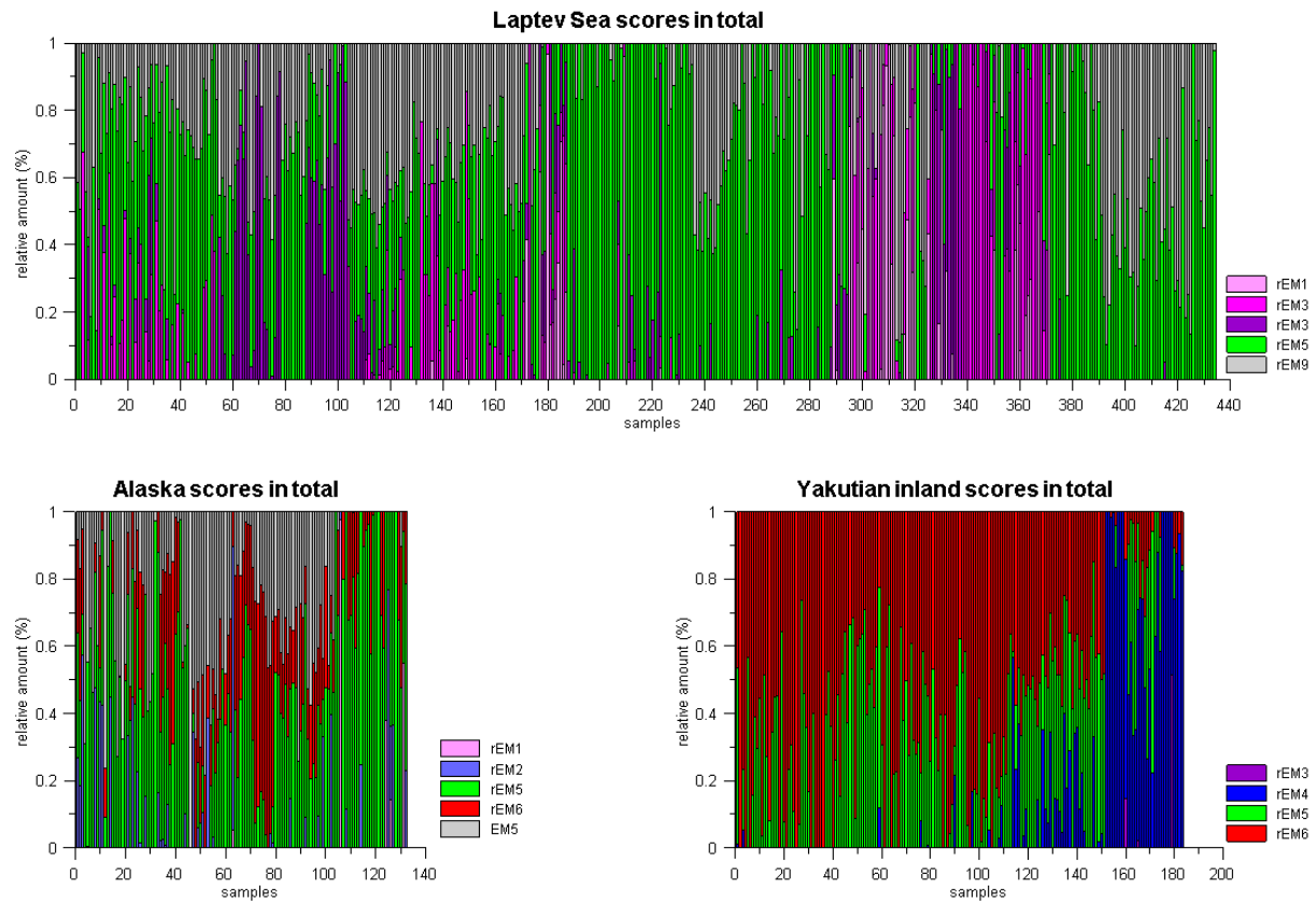
Fig. S6.2 The mean scores (the relative contribution of an endmember to each sample) for the three study regions. Please note, for better visual clarity loadings are not plotted with depth but in the same stratigraphic order.
